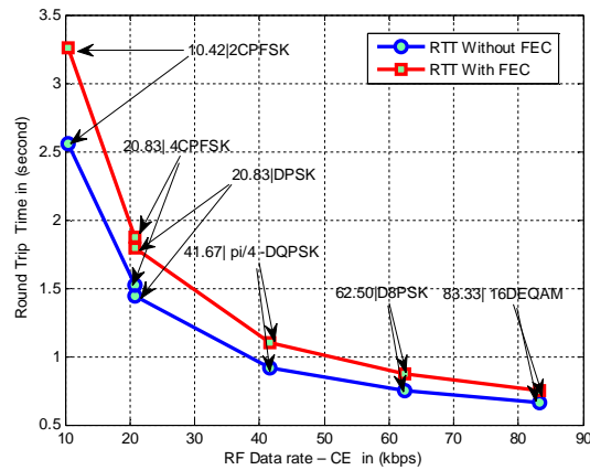
Figure 7. RTT versus RF data rates (kbps) for different modulation mode.
