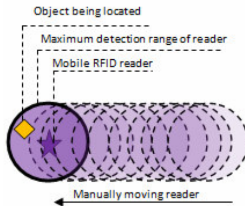
Figure 3. Proximity localisation using a mobile RFID Reader
