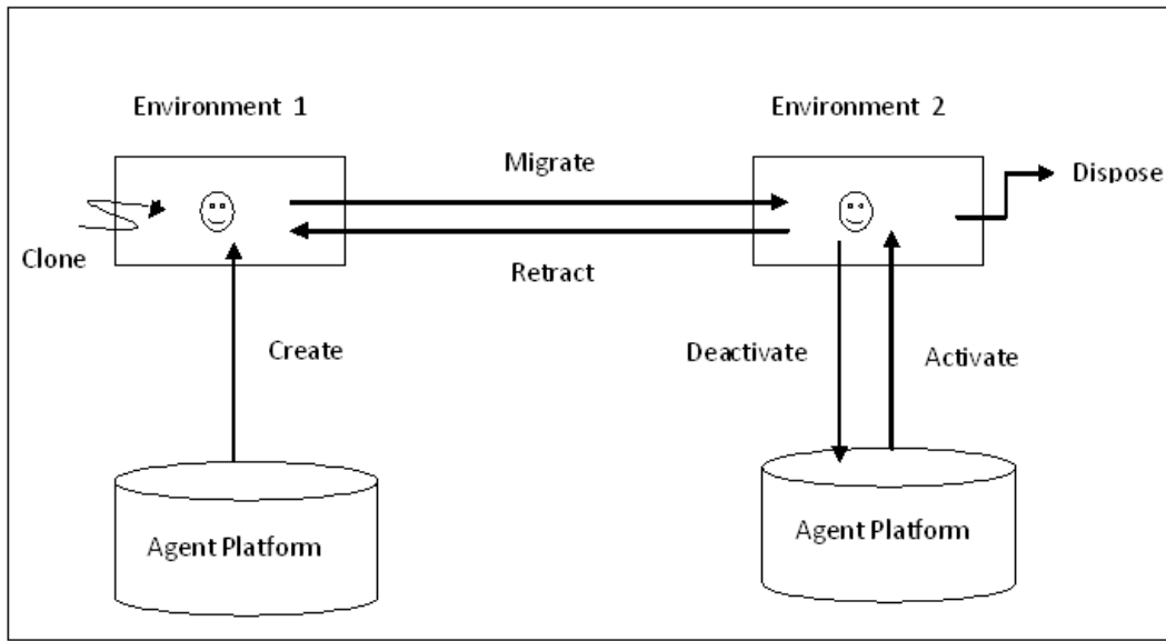
Fig. 4 Mobile Agent life cycle
