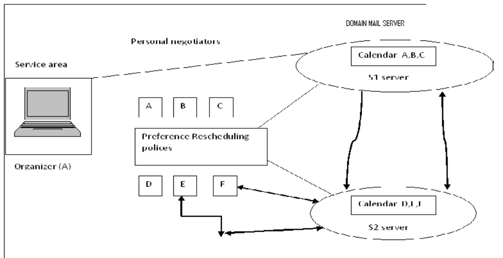
Fig 5. Mobile Agent Scheduler Scenario
