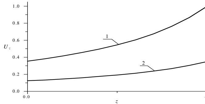
Fig. 8. Normalized dependences of component u_z of displacement vector on coordinate z for nonporous (curve 1) and porous (curve 2) epitaxial layers
