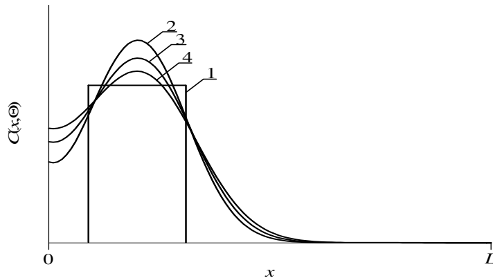
Fig. 5. Spatial distributions of dopant in heterostructure after ion implantation. Curve 1 is idealized distribution of dopant. Curves 2-4 are real distributions of dopant for different values of annealing time. Increasing of number of curve corresponds to increasing of annealing time
