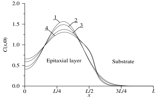
Fig.3. Distributions of concentration of implanted dopant in heterostructure from Fig. 1 in direction, which is perpendicular to interface between epitaxial layer substrate. Curves 1 and 3 corresponds to annealing time \Theta = 0.0048(L_x^2 + L_y^2 + L_z^2)/D_0 . Curves 2 and 4 corresponds to annealing time \Theta = 0.0057(L_x^2 + L_y^2 + L_z^2)/D_0 . Curves 1 and 2 corresponds to homogenous sample. Curves 3 and 4 corresponds to heterostructure under condition, when value of dopant diffusion coefficient in epitaxial layer is larger, than value of dopant diffusion coefficient in substrate
