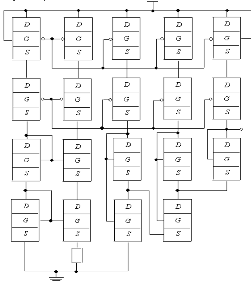
Fig. 1a. Structure of the considered voltage reference [20]
